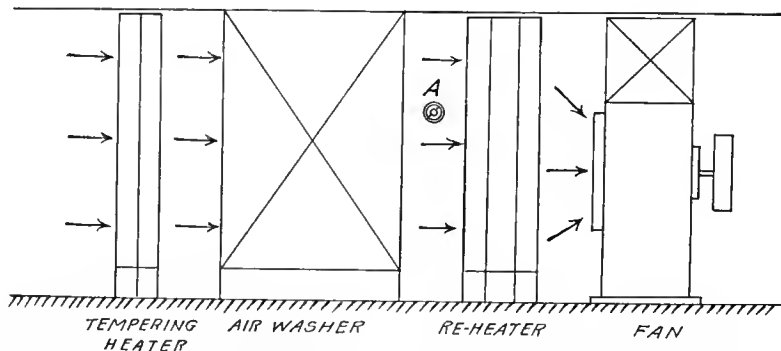
FIG. 9. DIAGRAM SHOWING ARRANGEMENT OF AIR WASHER IN RELATION TO THE FAN AND HEATERS
